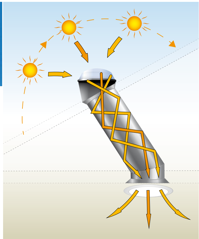
Light pipes scheme
