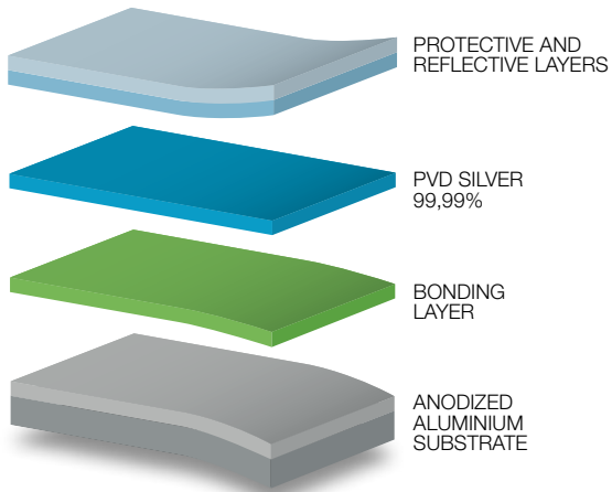
Coating System Diagram vega98
