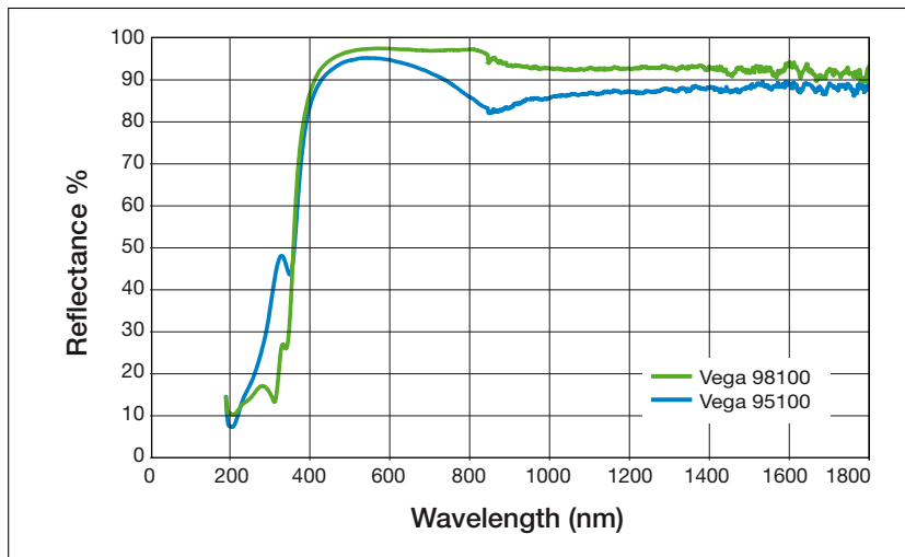
Comparison of spectral reflectance curves for Vega 98100 vs Vega 95100 and pre-anodized specular aluminium
